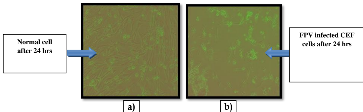
Fig. 5. a) Normal cell and b) FPV infected CEF cell after 24 hours of infection at 10x magnification
